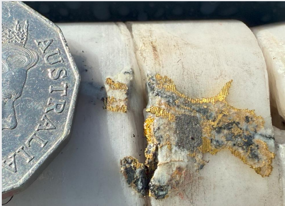
Visible gold in BMDD001W1 from 544.9m depth
