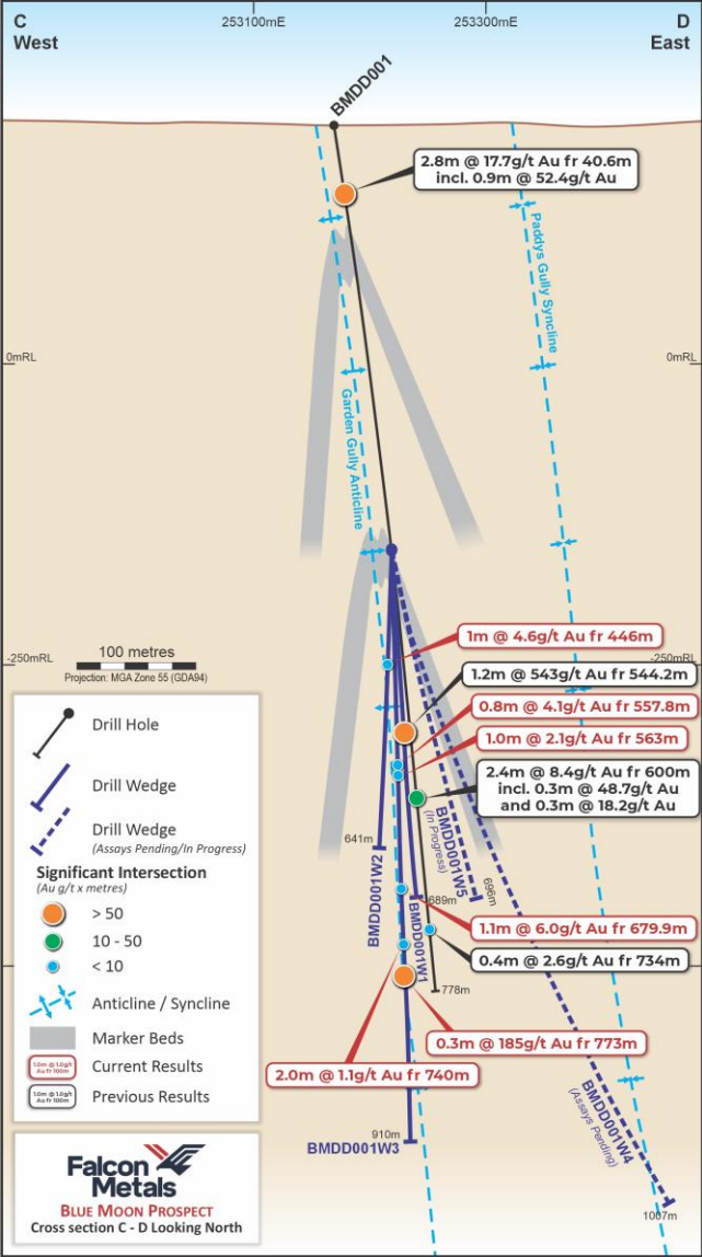
Cross section at Blue Moon
